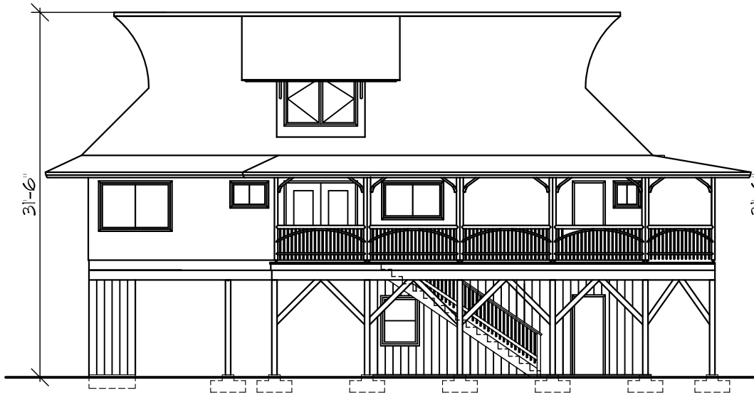
REAR ELEVATION
